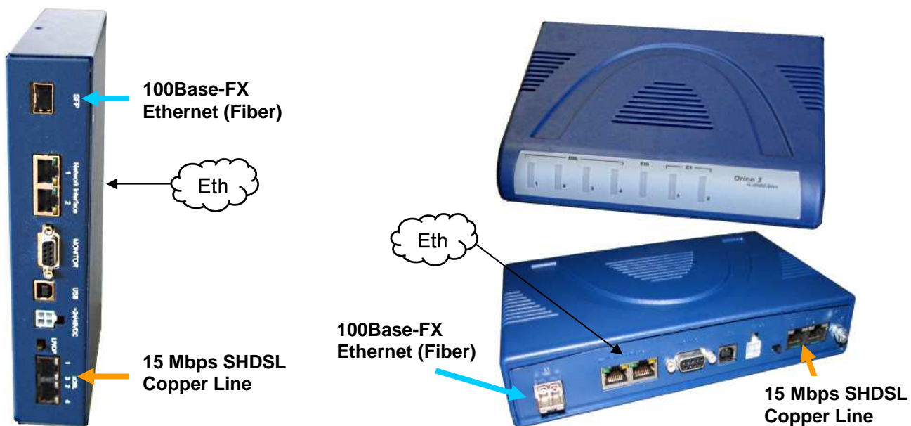
Picture 1.2: Orion3 (V84S) Dinrail Unit with Copper and Fiber Connection
