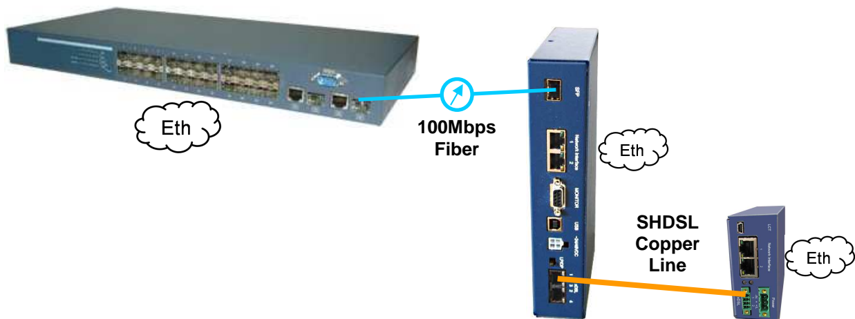
Application 2.4. Thrid Party Switch Connected to Orion3 or MiniFlex with 100Mbps
