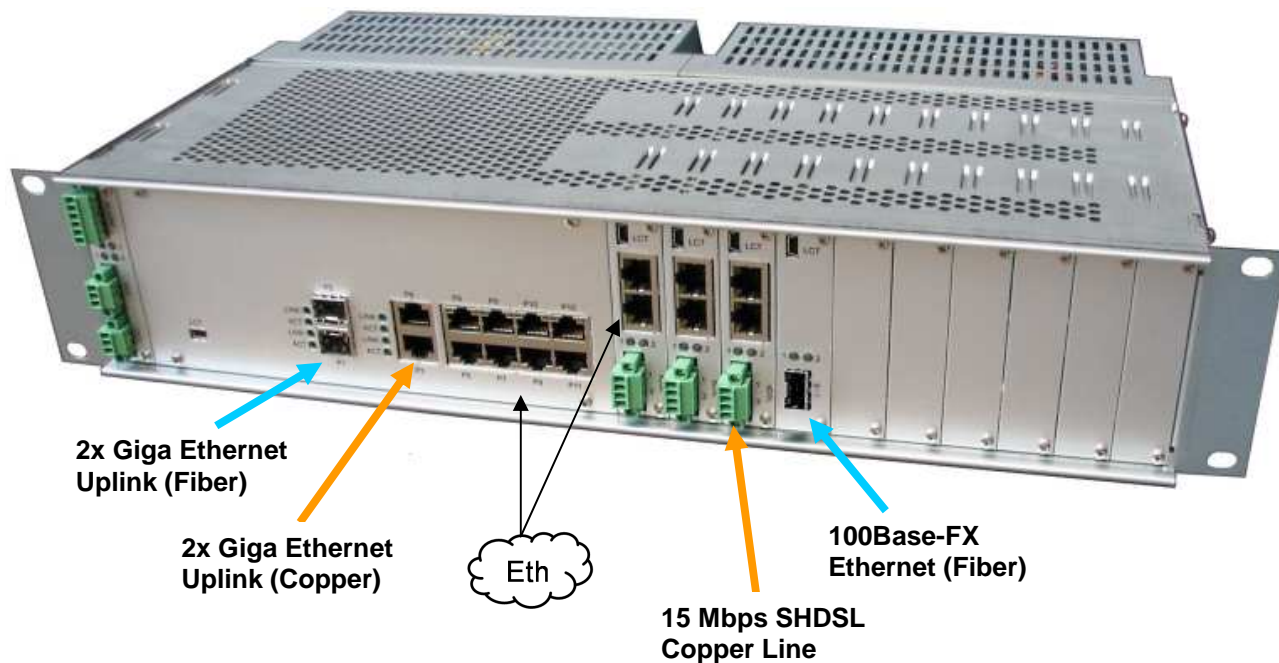
Picture 1.1: MiniFlex 19" 2U Minirack with Fiber & Copper Connections
