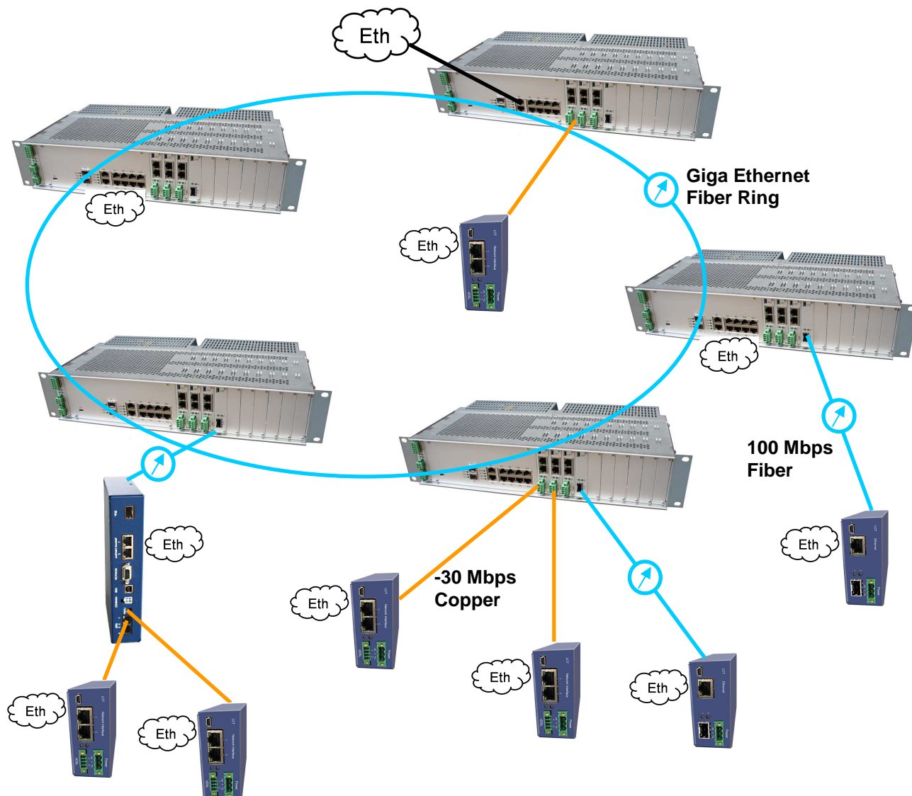
Application 2.1. Giga Fiber Ring and on each Station Fiber or Copper Connections
