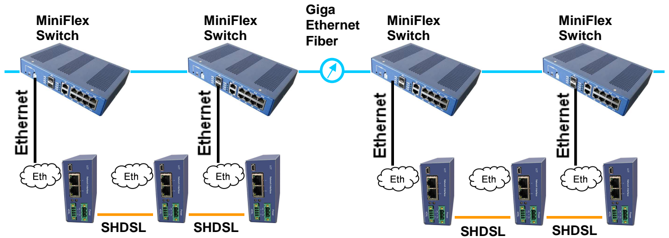
Application 2.2. Giga Fiber Bus and Ethernet Drop Insert in Ring Networks
