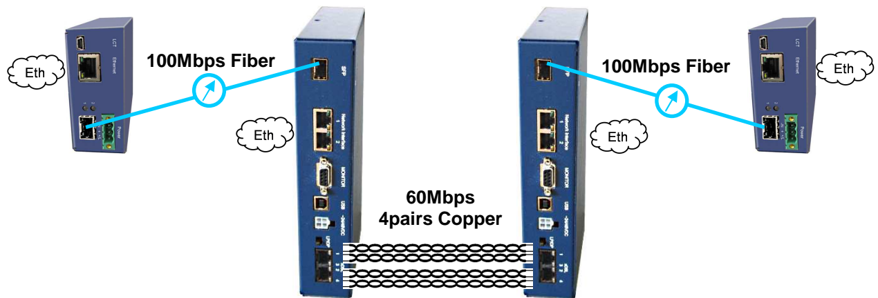
Application 2.3. 100Mbps Long Distance Copper to Fiber Converter
