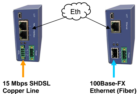
Picture 1.3: MiniFlex Dinrail Units with Copper or Fiber Connection
